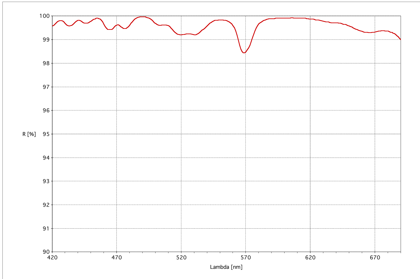
SHR Front Surface Mirror (SCALE of Y-axis is 90-100% ! ), 420-690nm
