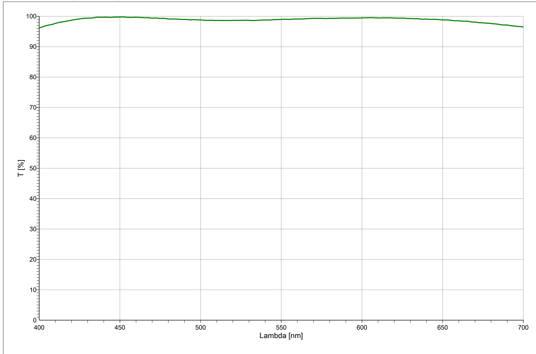
ARC-O Transmission, 400-700nm, Substratdicke: 3mm
